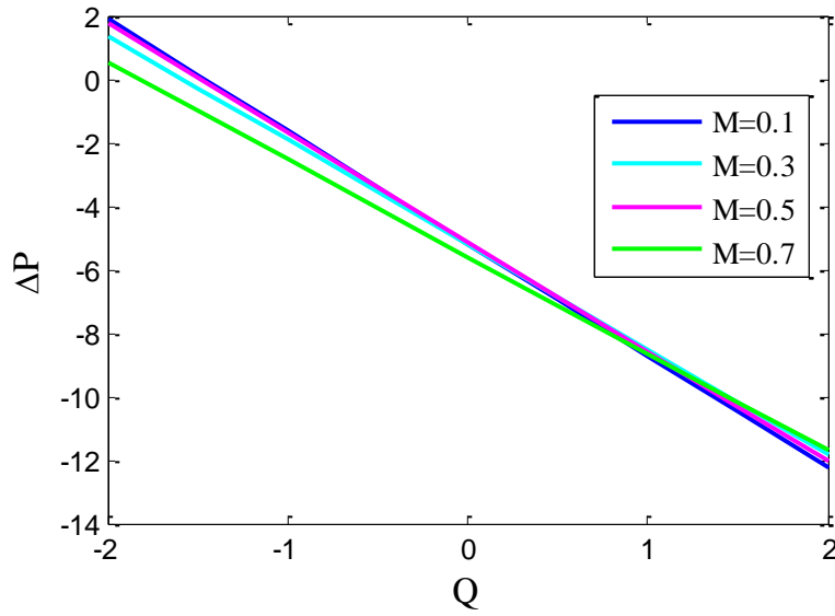
Fig.6. Pressure rise versus flow rate for different values for M .
