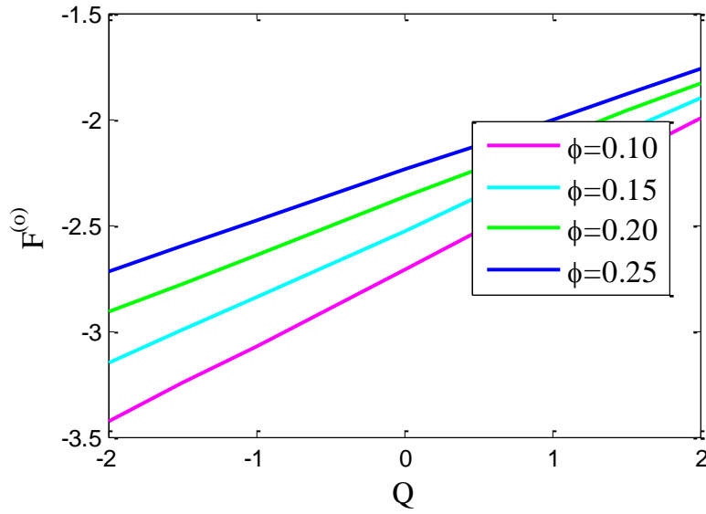
Fig.8. Frictional force on inner tube versus flow rate for different values for \phi .
