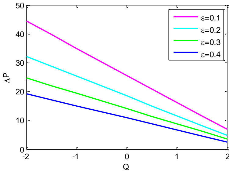
Fig.4. Pressure rise versus flow rate for different values for \epsilon .
