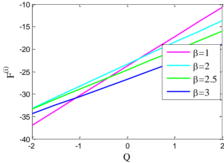
Fig.15. Frictional force on outer tube versus flow rate for different values for \beta .
