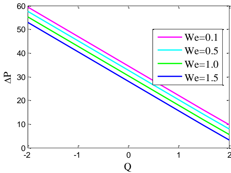
Fig.2. Pressure rise versus flow rate for different values for We
