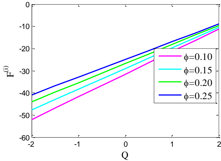
Fig.13. Frictional force on outer tube versus flow rate for different values for \phi .
