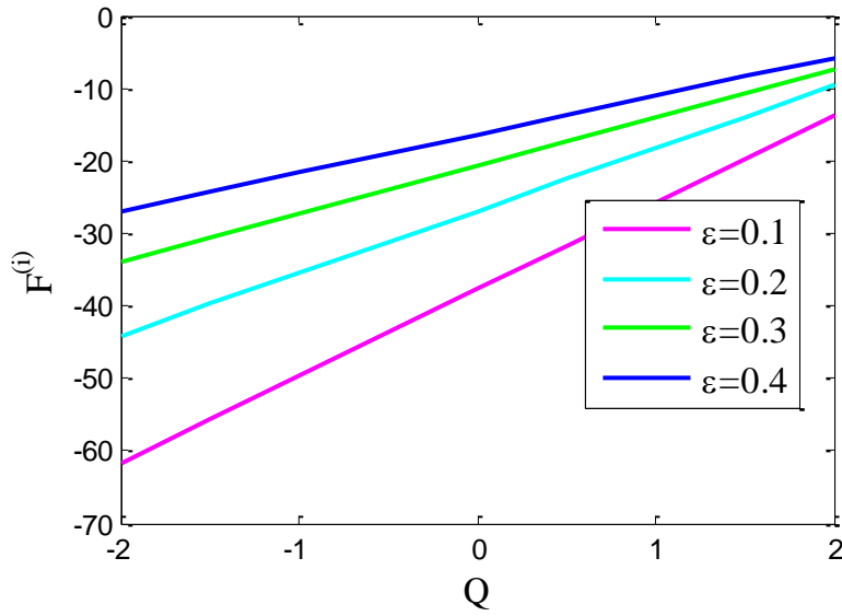
Fig.14. Frictional force on outer tube versus flow rate for different values for \epsilon .
