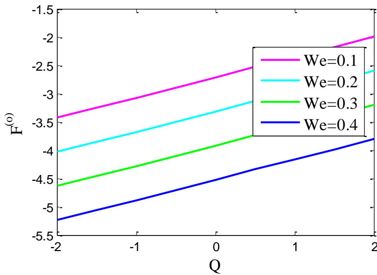
Fig.7. Frictional force on inner tube versus flow rate for different values for We .
