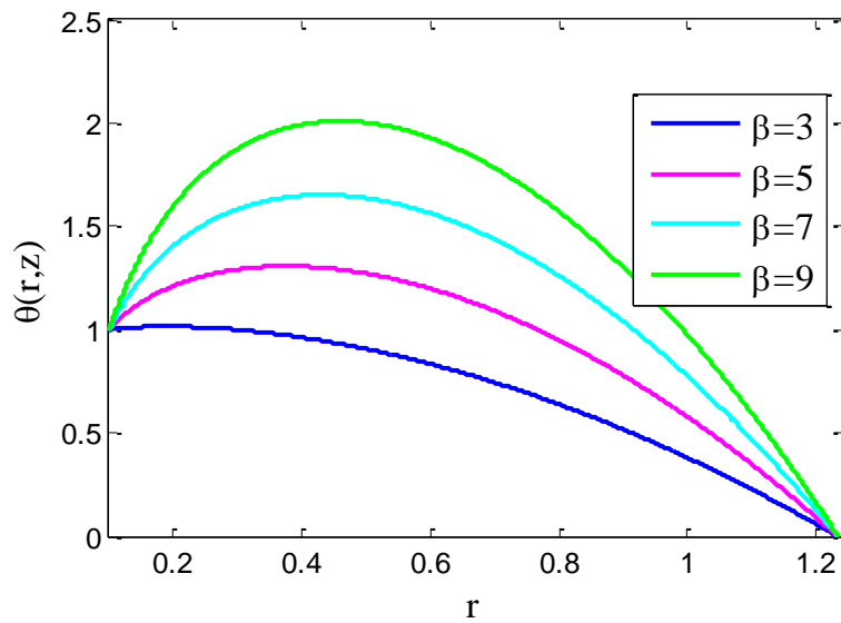
Fig.17. Plot for Temperature field for different values for \beta .
