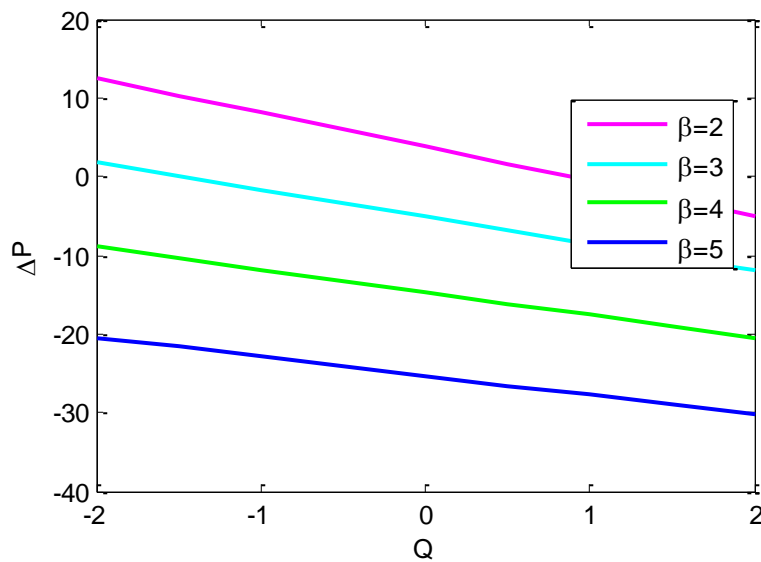
Fig.5. Pressure rise versus flow rate for different values for \beta .
