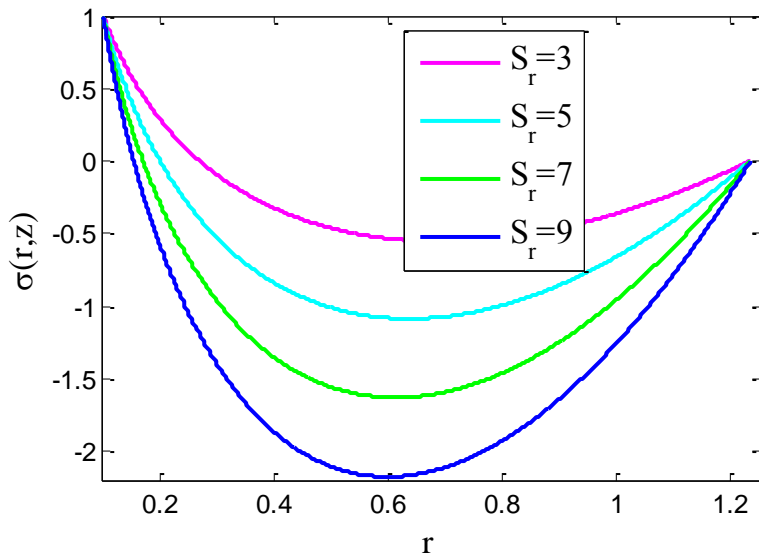
Fig.19. Plot for Concentration for different values for Sr .
