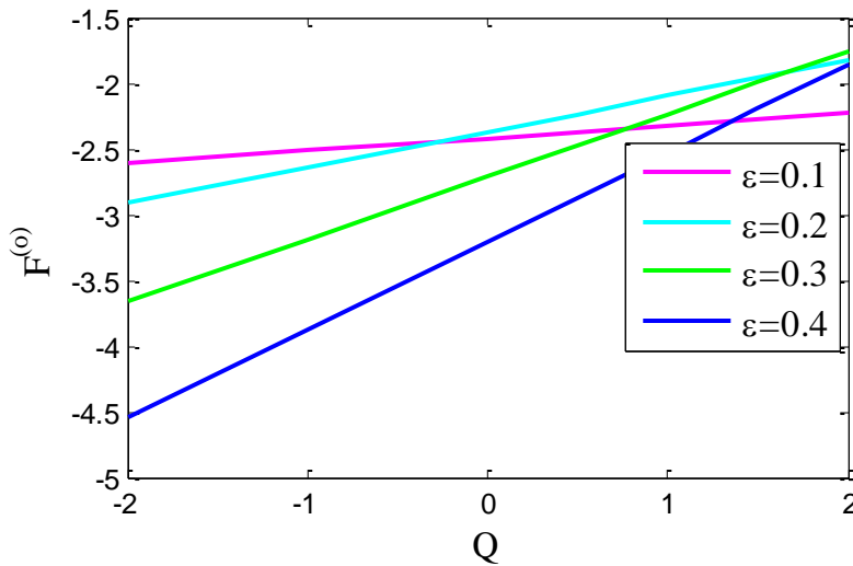
Fig.9. Frictional force on inner tube versus flow rate for different values for \epsilon .
