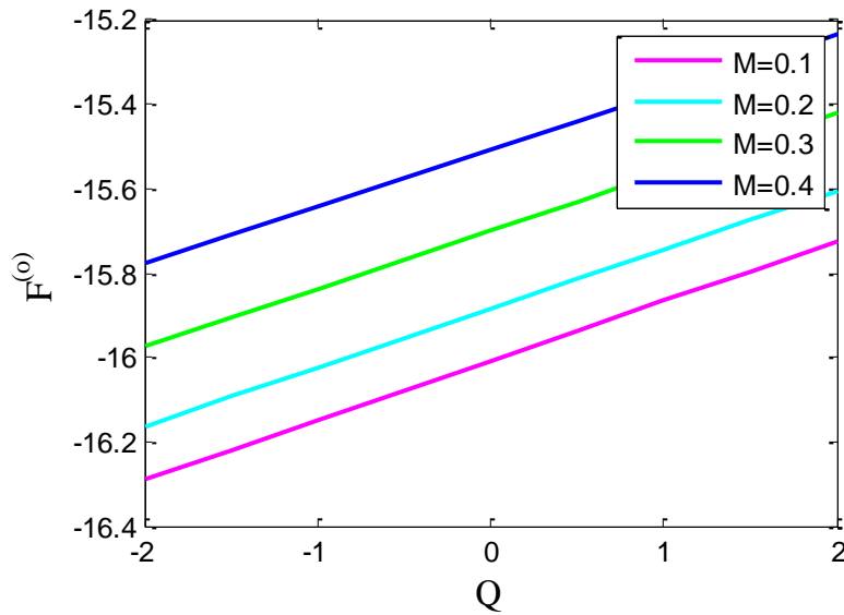
Fig.11. Frictional force on inner tube versus flow rate for different values for M .
