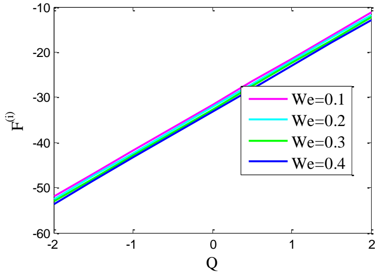
Fig.12. Frictional force on outer tube versus flow rate for different values for We .
